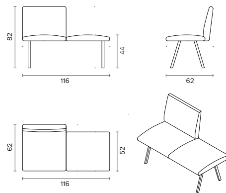
DOUBLE WITH SINGLE BACK RIGHT - L21R
