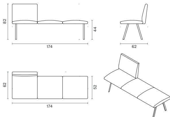
TRIPLE WITH SINGLE BACK RIGHT - L31R
