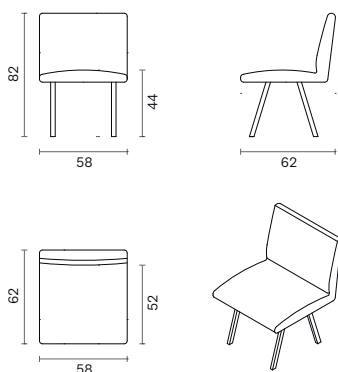
SINGLE WITH BACK - L1B
