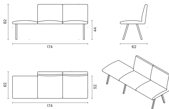
TRIPLE WITH DOUBLE BACK LEFT - L32L
