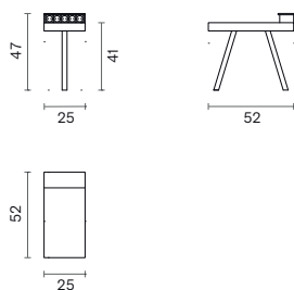
SIDE TABLE WITH PLUG - LC2
