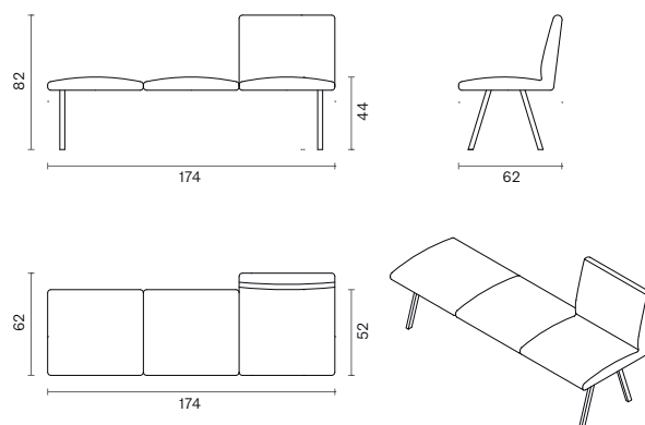
TRIPLE WITH SINGLE BACK LEFT - L31L
