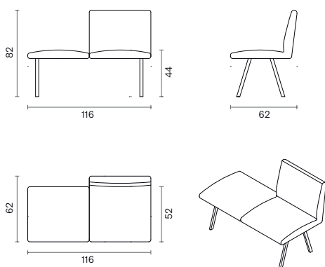
DOUBLE WITH SINGLE BACK LEFT - L21L
