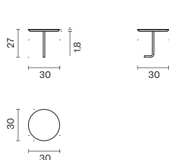
BENCH ROUND TABLE - LC1
