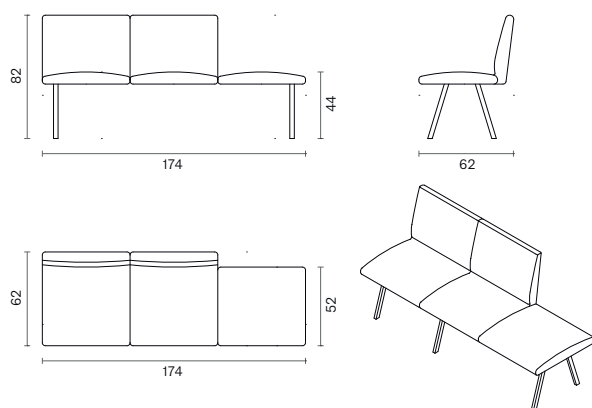
TRIPLE WITH DOUBLE BACK RIGHT - L32R
